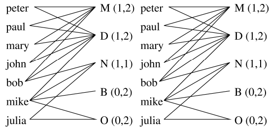
Figure 4.2. An example of a global cardinality constraint.
